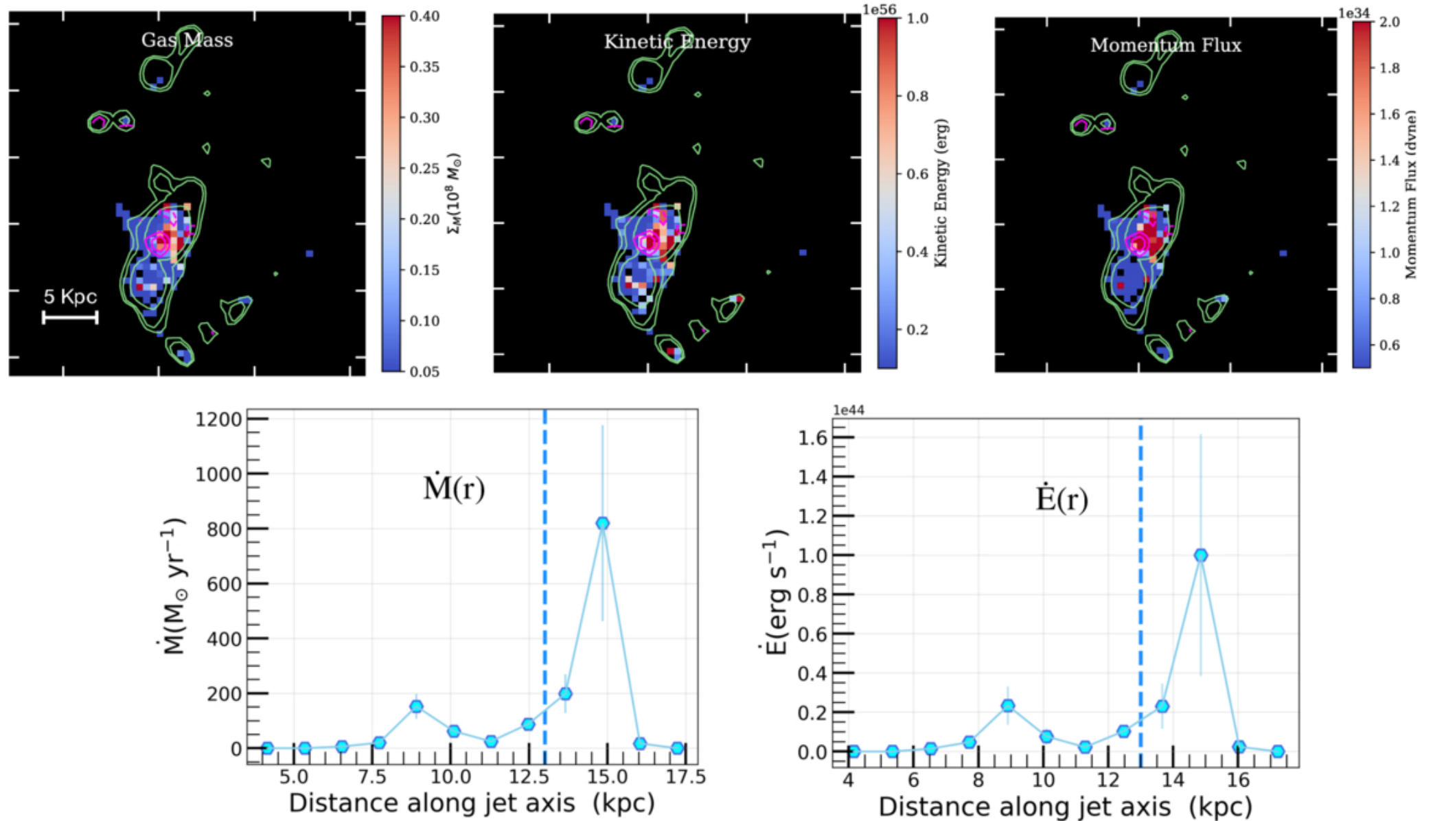
Figure 12. from Namrata Roy et al 2026 Astrophys. J. 1002 doi:10.3847/1538-4357/ae5b68 https://dx.doi.org/10.3847/1538-4357/ae5b68 © 2026. The Author(s). Published by the American Astronomical Society.
