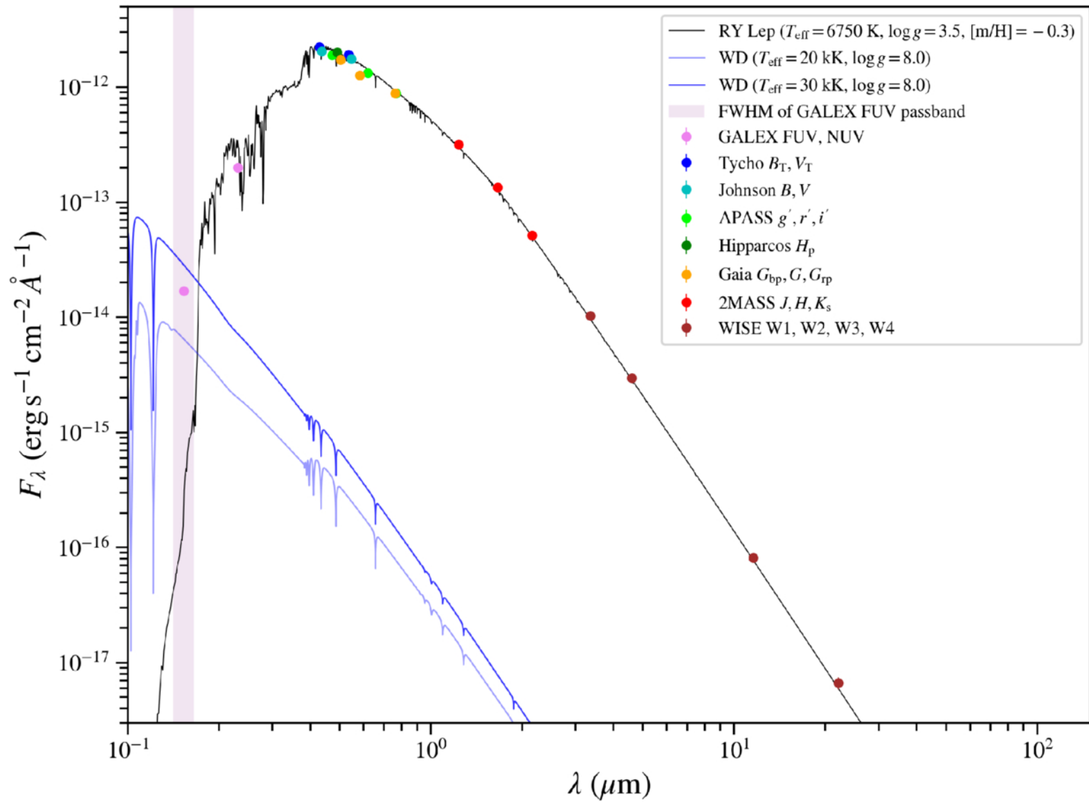
Figure 7. from Wojciech Niewiadomski et al 2026 Astrophys. J. 1002 doi:10.3847/1538-4357/ae5a95 https://dx.doi.org/10.3847/1538-4357/ae5a95 © 2026. The Author(s). Published by the American Astronomical Society.
