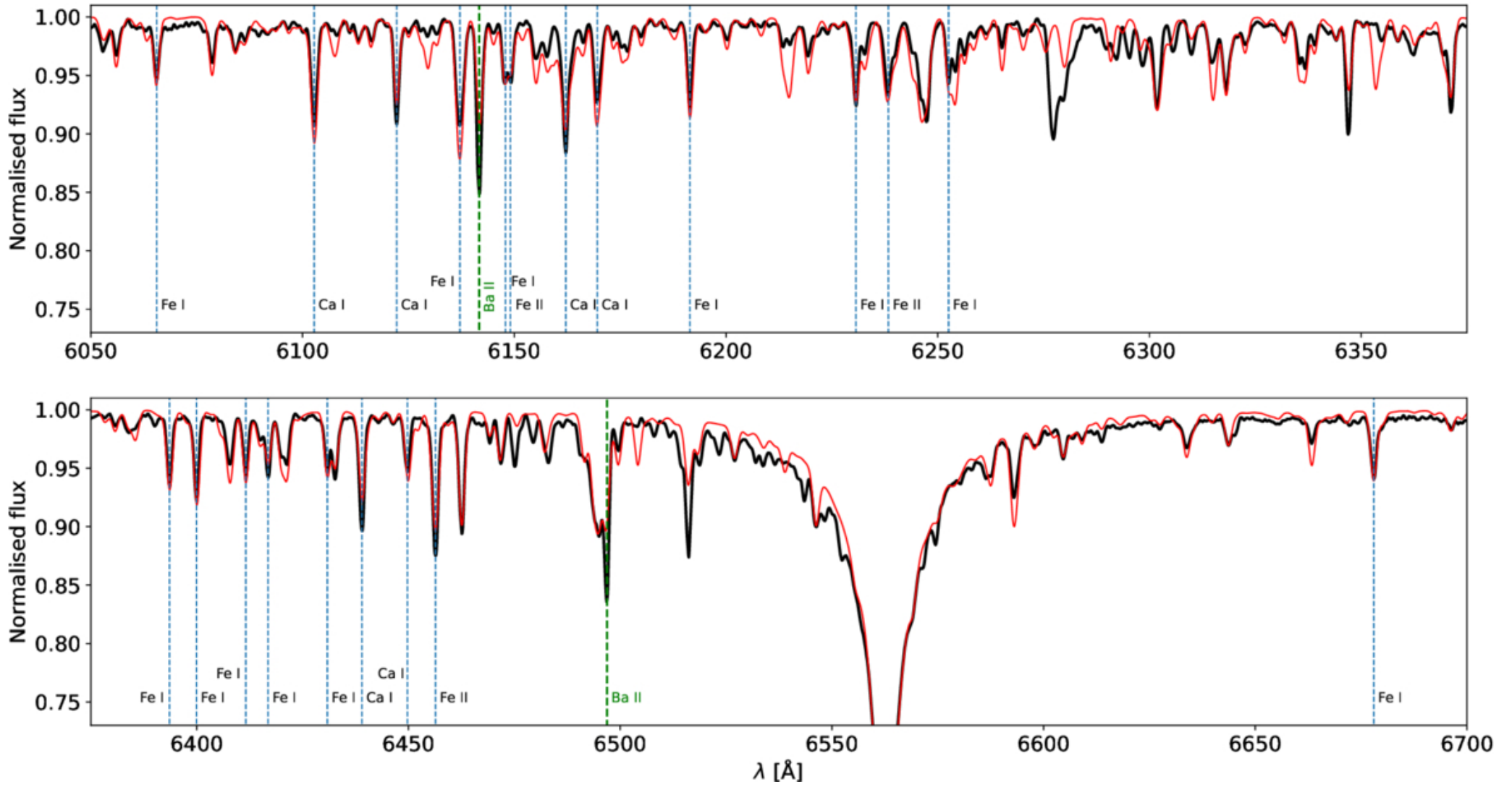
Figure 5. from Wojciech Niewiadomski et al 2026 Astrophys. J. 1002 doi:10.3847/1538-4357/ae5a95 https://dx.doi.org/10.3847/1538-4357/ae5a95 © 2026. The Author(s). Published by the American Astronomical Society.
