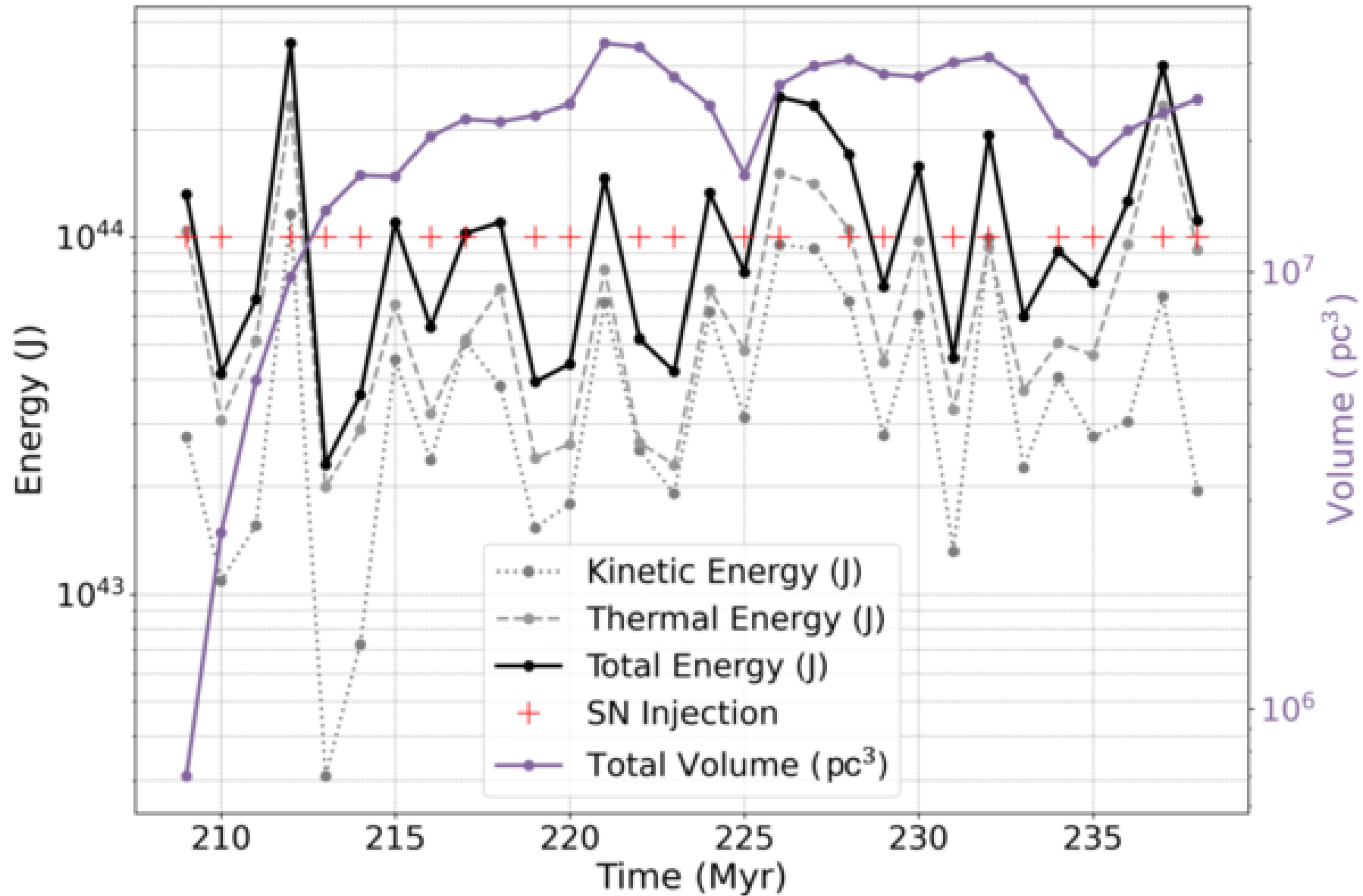
Figure 8. from Jing-Wen Chen et al 2026 Astrophys. J. 1004 doi:10.3847/1538-4357/ae5a26 https://dx.doi.org/10.3847/1538-4357/ae5a26 © 2026. The Author(s). Published by the American Astronomical Society.
