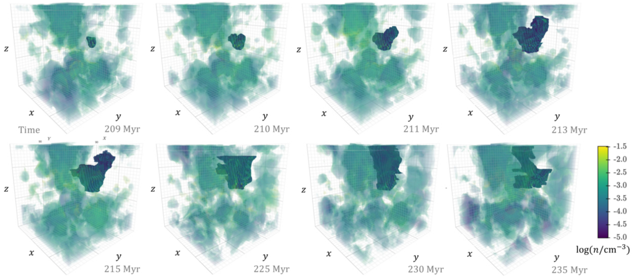
Figure 7. from Jing-Wen Chen et al 2026 Astrophys. J. 1004 doi:10.3847/1538-4357/ae5a26 https://dx.doi.org/10.3847/1538-4357/ae5a26 © 2026. The Author(s). Published by the American Astronomical Society.
