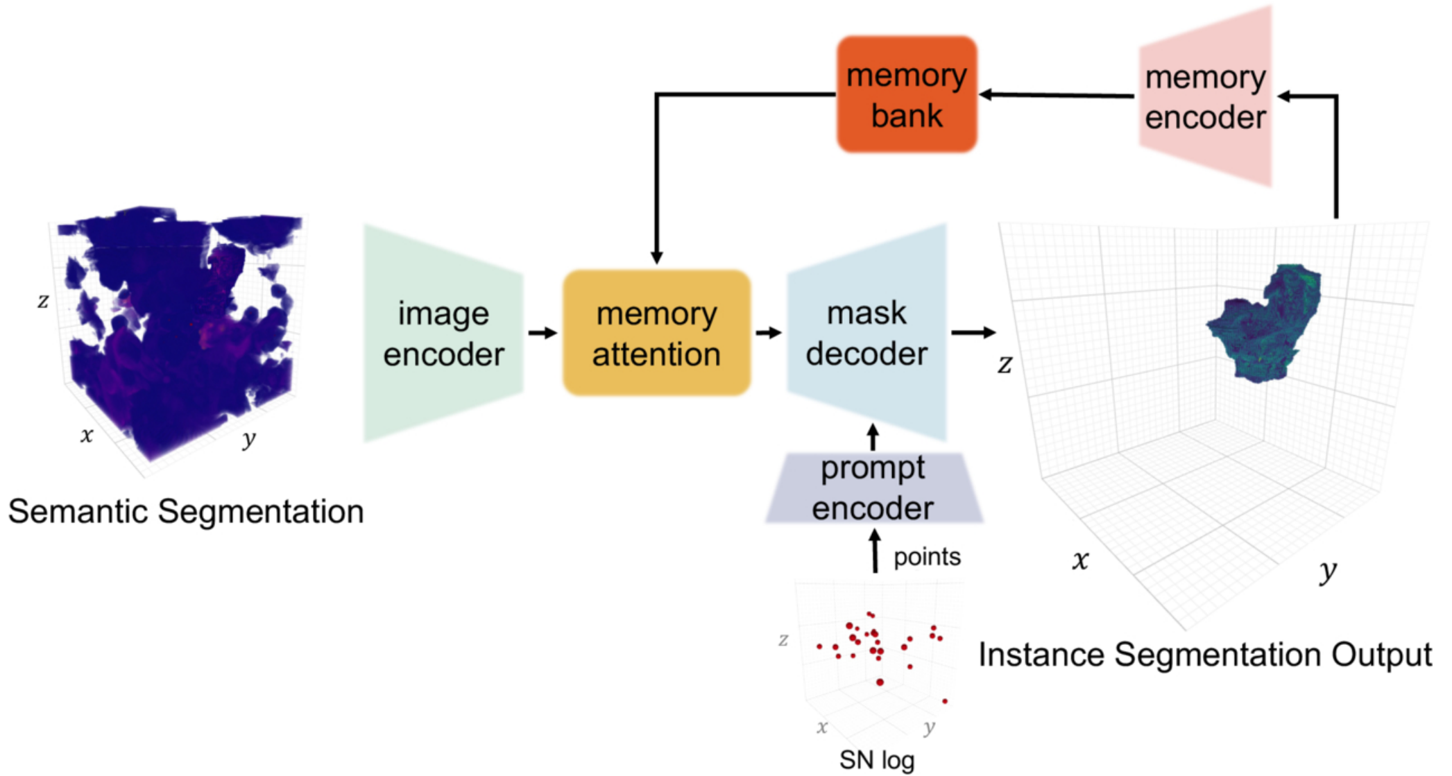
Figure 5. from Jing-Wen Chen et al 2026 Astrophys. J. 1004 doi:10.3847/1538-4357/ae5a26 https://dx.doi.org/10.3847/1538-4357/ae5a26 © 2026. The Author(s). Published by the American Astronomical Society.
