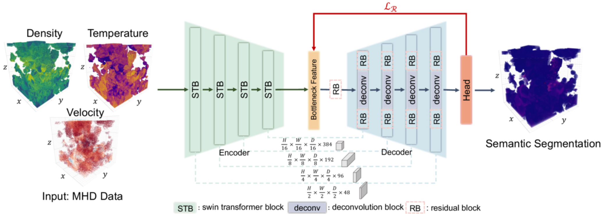
Figure 4. from Jing-Wen Chen et al 2026 Astrophys. J. 1004 doi:10.3847/1538-4357/ae5a26 https://dx.doi.org/10.3847/1538-4357/ae5a26 © 2026. The Author(s). Published by the American Astronomical Society.
