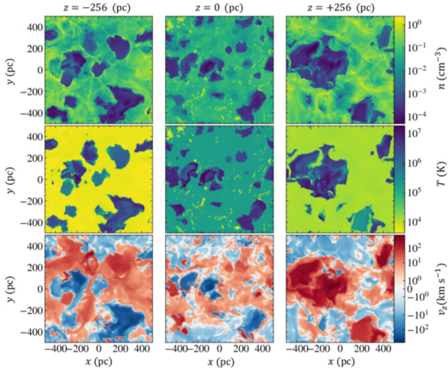
Figure 2. from Jing-Wen Chen et al 2026 Astrophys. J. 1004 doi:10.3847/1538-4357/ae5a26 https://dx.doi.org/10.3847/1538-4357/ae5a26 © 2026. The Author(s). Published by the American Astronomical Society.
