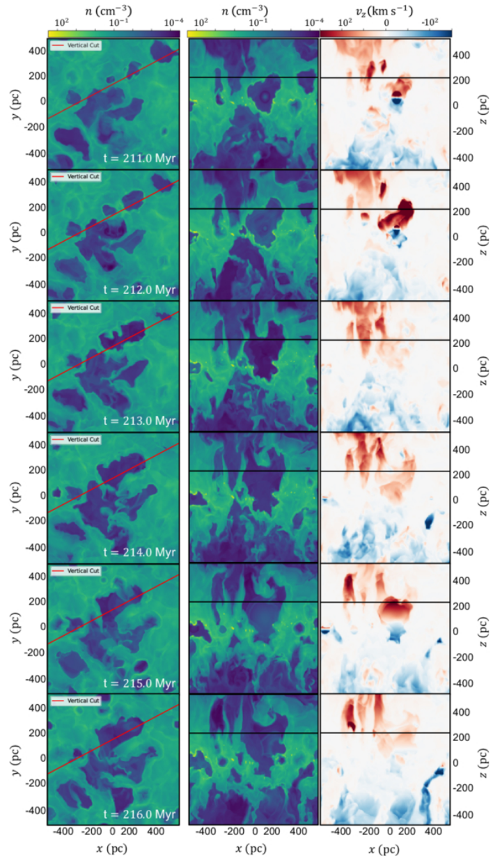
Figure 10. from Jing-Wen Chen et al 2026 Astrophys. J. 1004 doi:10.3847/1538-4357/ae5a26 https://dx.doi.org/10.3847/1538-4357/ae5a26 © 2026. The Author(s). Published by the American Astronomical Society.
