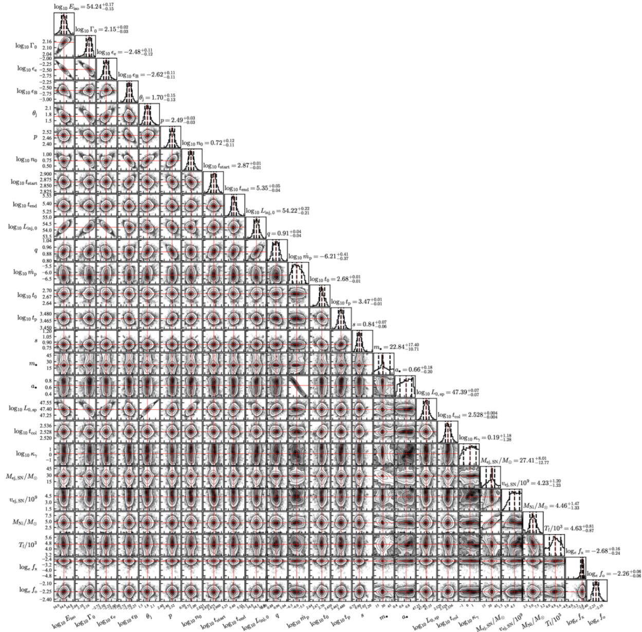
Figure 5. from Liang-Jun Chen et al 2026 Astrophys. J. 1002 doi:10.3847/1538-4357/ae595e https://dx.doi.org/10.3847/1538-4357/ae595e © 2026. The Author(s). Published by the American Astronomical Society.
