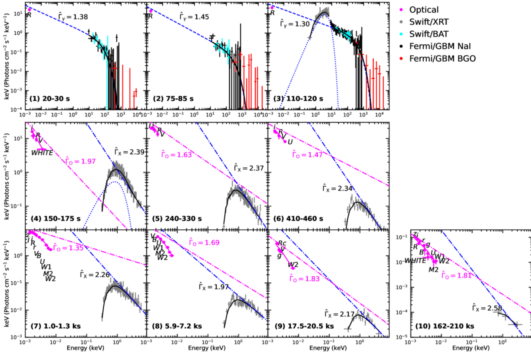
Figure 3. from Liang-Jun Chen et al 2026 Astrophys. J. 1002 doi:10.3847/1538-4357/ae595e https://dx.doi.org/10.3847/1538-4357/ae595e © 2026. The Author(s). Published by the American Astronomical Society.
