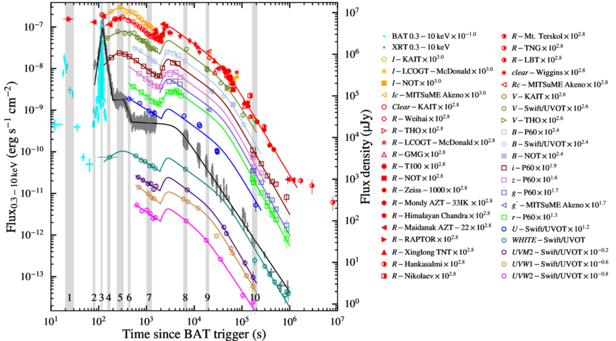
Figure 1. from Liang-Jun Chen et al 2026 Astrophys. J. 1002 doi:10.3847/1538-4357/ae595e https://dx.doi.org/10.3847/1538-4357/ae595e © 2026. The Author(s). Published by the American Astronomical Society.
