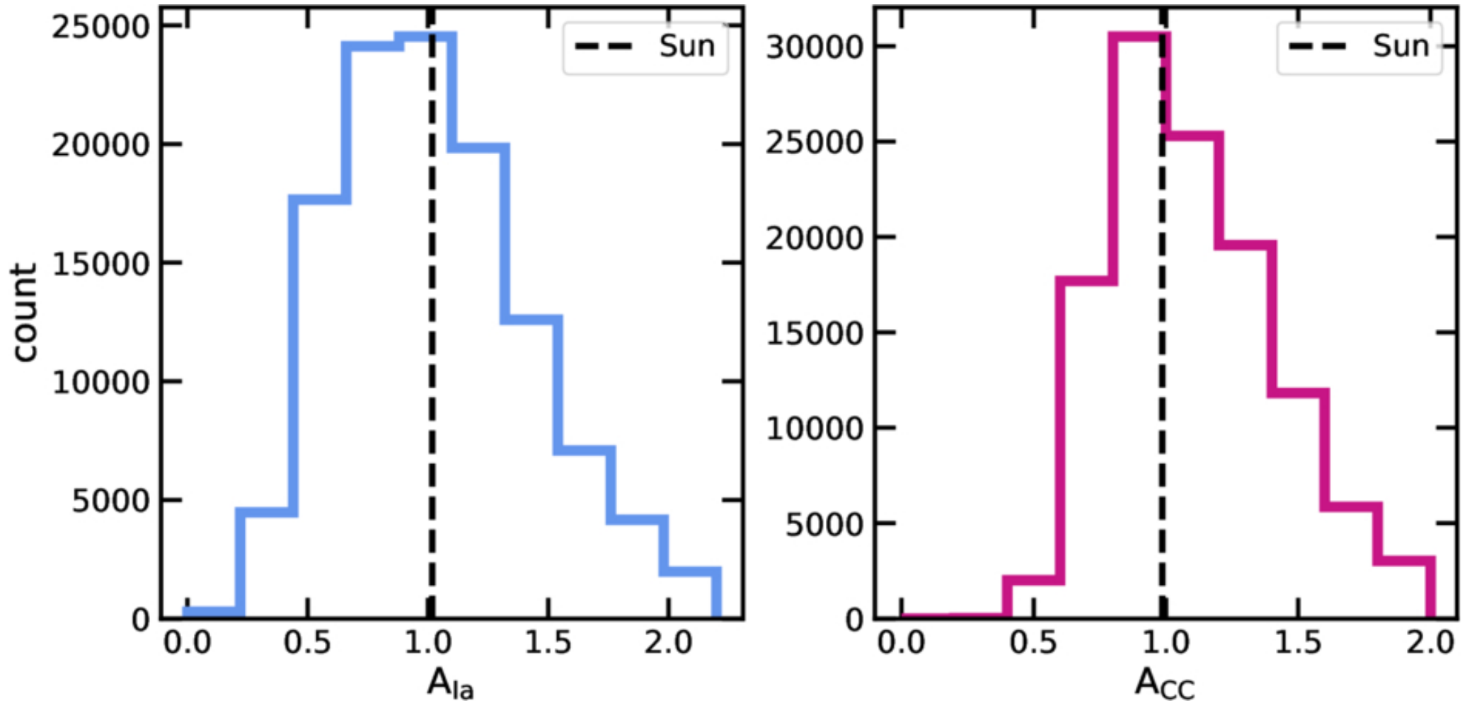
Figure 8. from Rayna Rampalli et al 2026 Astrophys. J. 1002 doi:10.3847/1538-4357/ae5955 https://dx.doi.org/10.3847/1538-4357/ae5955 © 2026. The Author(s). Published by the American Astronomical Society.
