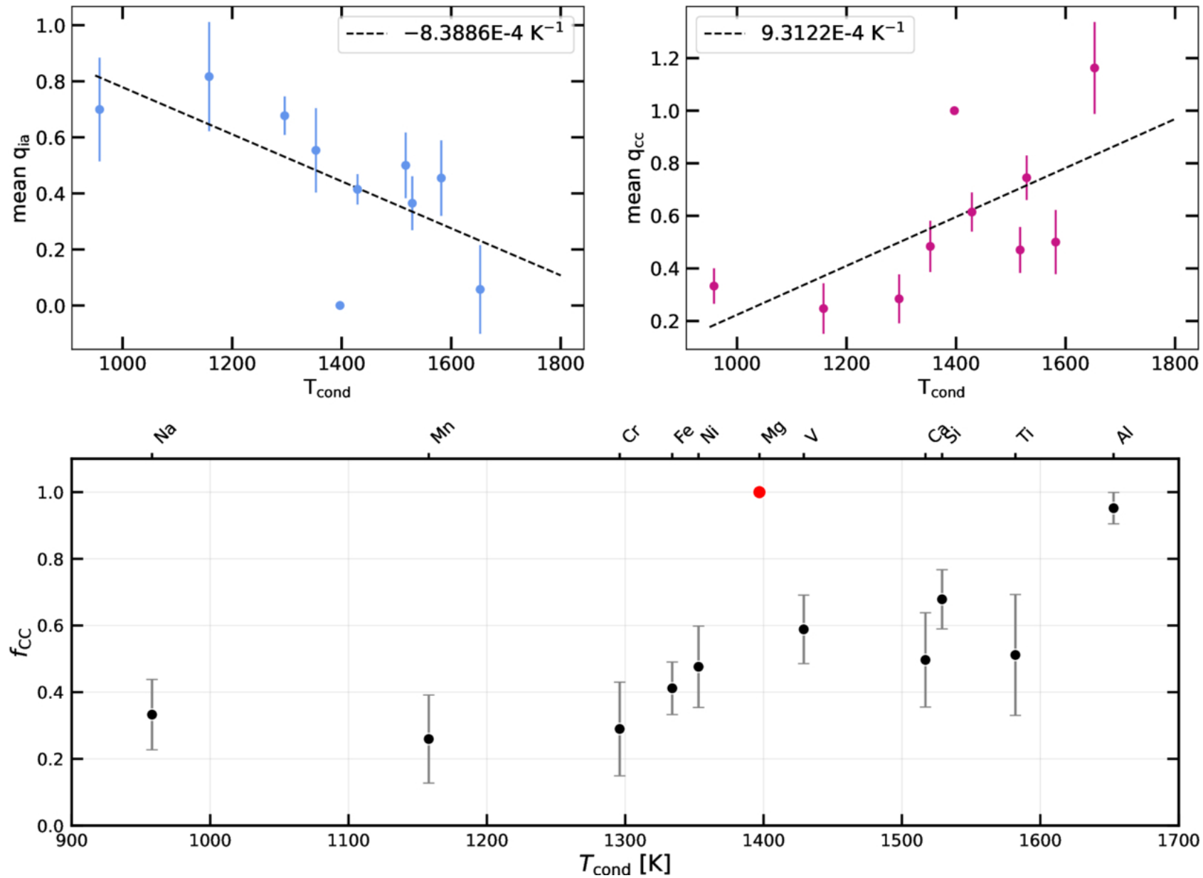
Figure 10. from Rayna Rampalli et al 2026 Astrophys. J. 1002 doi:10.3847/1538-4357/ae5955 https://dx.doi.org/10.3847/1538-4357/ae5955 © 2026. The Author(s). Published by the American Astronomical Society.
