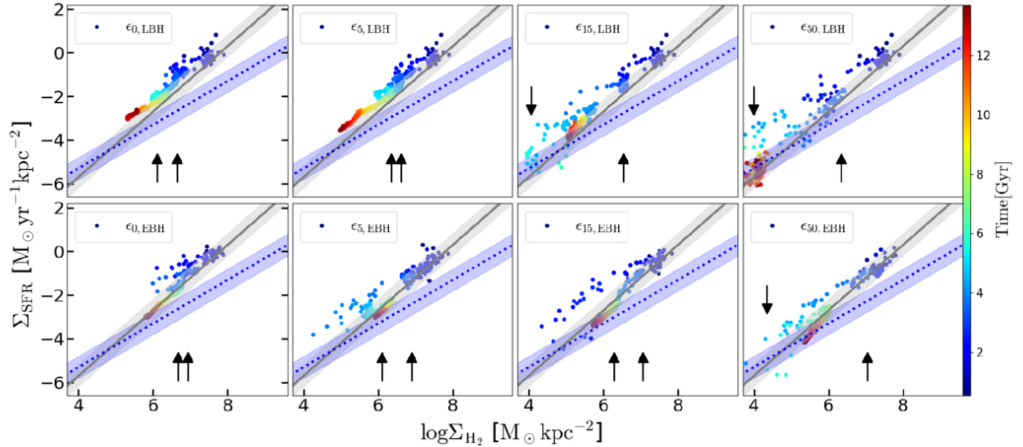
Figure 5. from Julianne Goddard et al 2026 Astrophys. J. 1001 doi:10.3847/1538-4357/ae5939 https://dx.doi.org/10.3847/1538-4357/ae5939 © 2026. The Author(s). Published by the American Astronomical Society.
