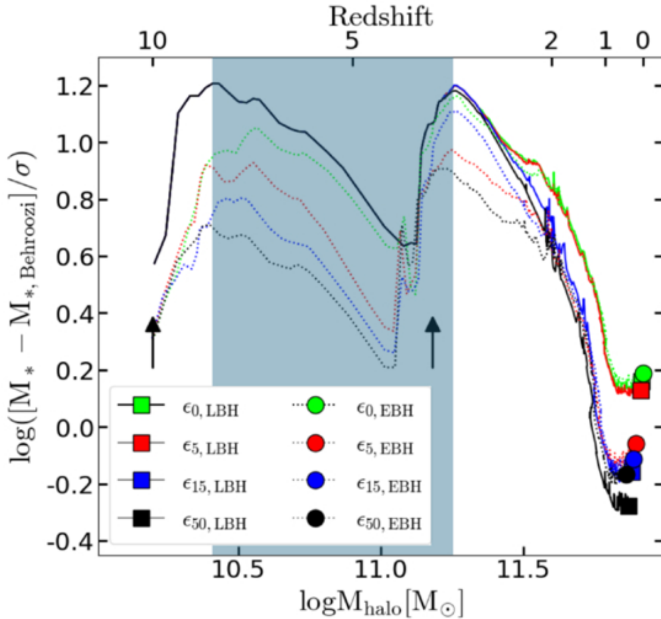
Figure 2. from Julianne Goddard et al 2026 Astrophys. J. 1001 doi:10.3847/1538-4357/ae5939 https://dx.doi.org/10.3847/1538-4357/ae5939 © 2026. The Author(s). Published by the American Astronomical Society.
