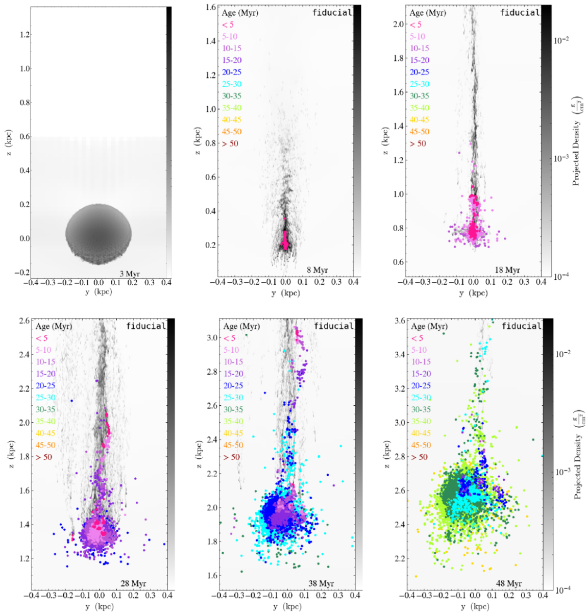
Figure 4. from Stephanie Tonnesen et al 2026 Astrophys. J. 1002 doi:10.3847/1538-4357/ae5937 https://dx.doi.org/10.3847/1538-4357/ae5937 © 2026. The Author(s). Published by the American Astronomical Society.
