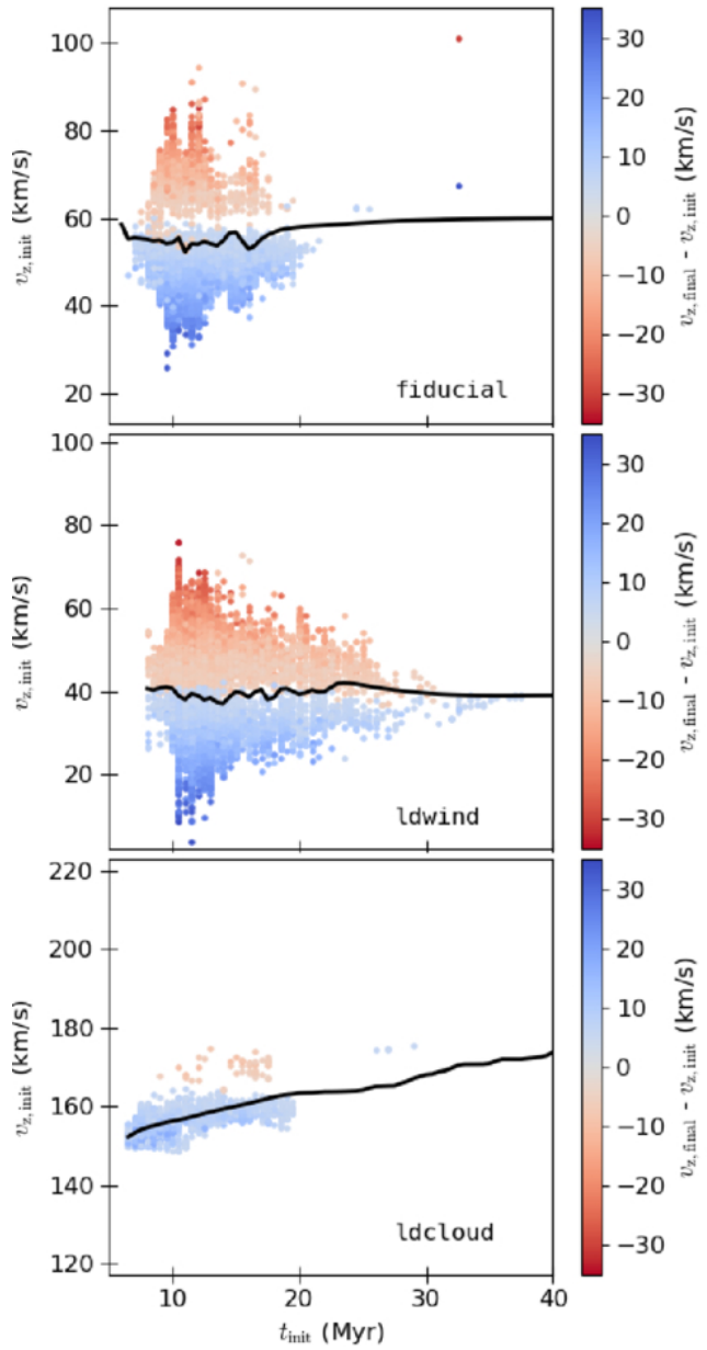
Figure 11. from Stephanie Tonnesen et al 2026 Astrophys. J. 1002 doi:10.3847/1538-4357/ae5937 https://dx.doi.org/10.3847/1538-4357/ae5937 © 2026. The Author(s). Published by the American Astronomical Society.
