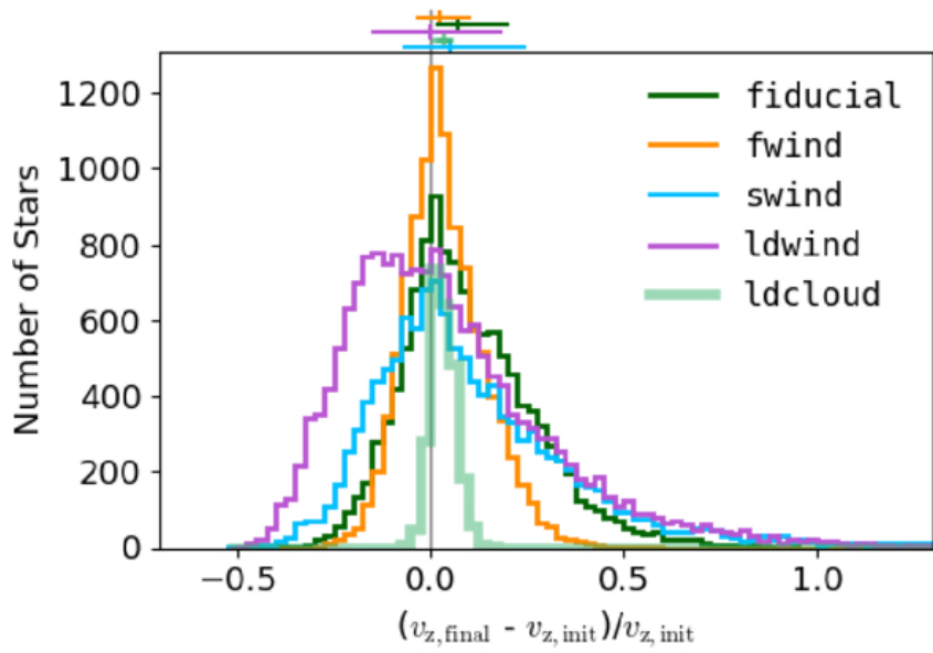
Figure 10. from Stephanie Tonnesen et al 2026 Astrophys. J. 1002 doi:10.3847/1538-4357/ae5937 https://dx.doi.org/10.3847/1538-4357/ae5937 © 2026. The Author(s). Published by the American Astronomical Society.
