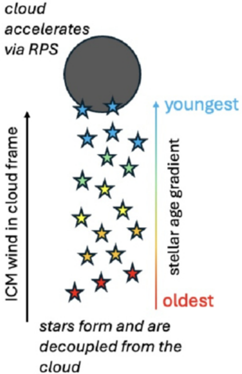
Figure 1. from Stephanie Tonnesen et al 2026 Astrophys. J. 1002 doi:10.3847/1538-4357/ae5937 https://dx.doi.org/10.3847/1538-4357/ae5937 © 2026. The Author(s). Published by the American Astronomical Society.
