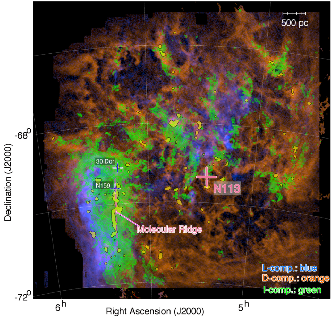
Figure A1. from Rin I. Yamada et al 2026 Astrophys. J. 1003 doi:10.3847/1538-4357/ae58ab https://dx.doi.org/10.3847/1538-4357/ae58ab © 2026. The Author(s). Published by the American Astronomical Society.
