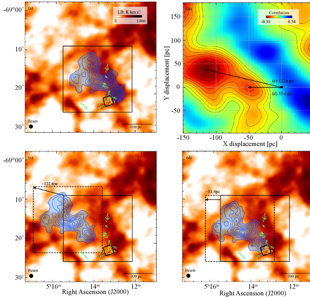
Figure 7. from Rin I. Yamada et al 2026 Astrophys. J. 1003 doi:10.3847/1538-4357/ae58ab https://dx.doi.org/10.3847/1538-4357/ae58ab © 2026. The Author(s). Published by the American Astronomical Society.
