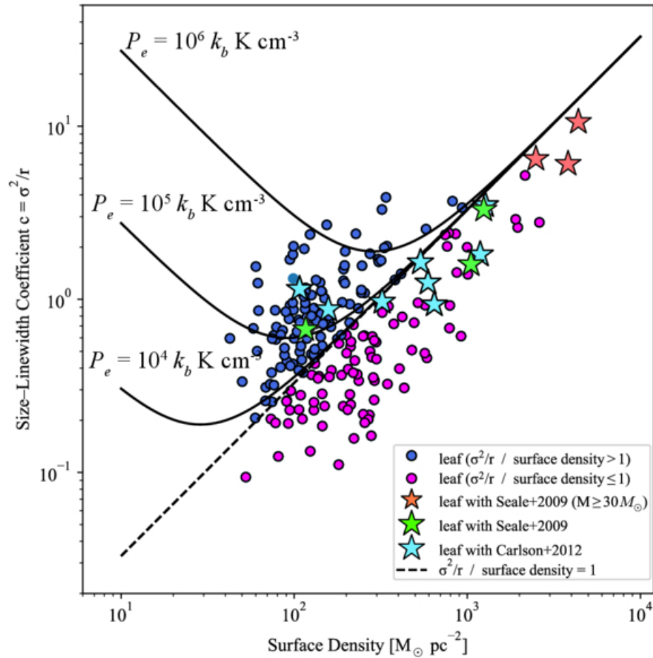
Figure 4. from Rin I. Yamada et al 2026 Astrophys. J. 1003 doi:10.3847/1538-4357/ae58ab https://dx.doi.org/10.3847/1538-4357/ae58ab © 2026. The Author(s). Published by the American Astronomical Society.
