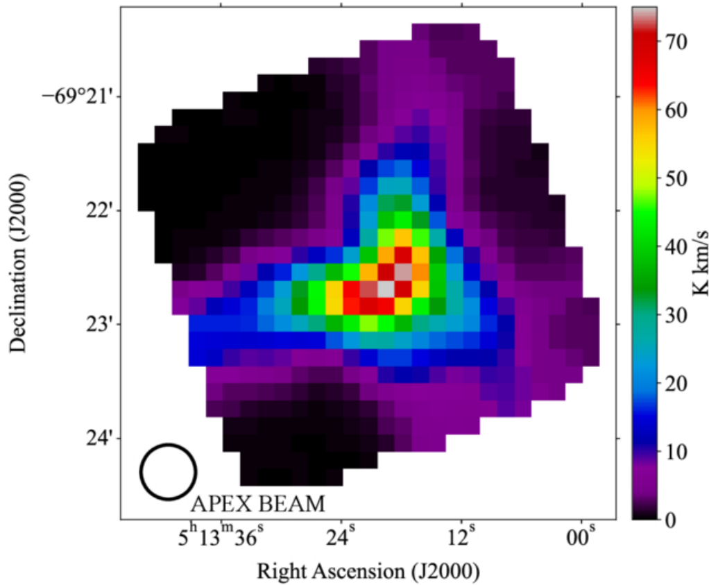
(a) APEX CO(J=2-1)
