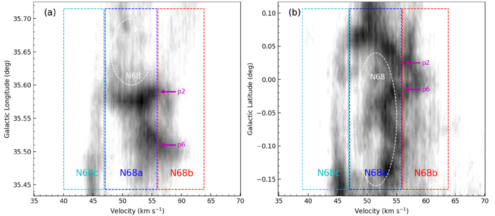
Figure 8. from En Chen and Xi Chen 2026 Astrophys. J. 1001 doi:10.3847/1538-4357/ae58a6 https://dx.doi.org/10.3847/1538-4357/ae58a6 © 2026. The Author(s). Published by the American Astronomical Society.
