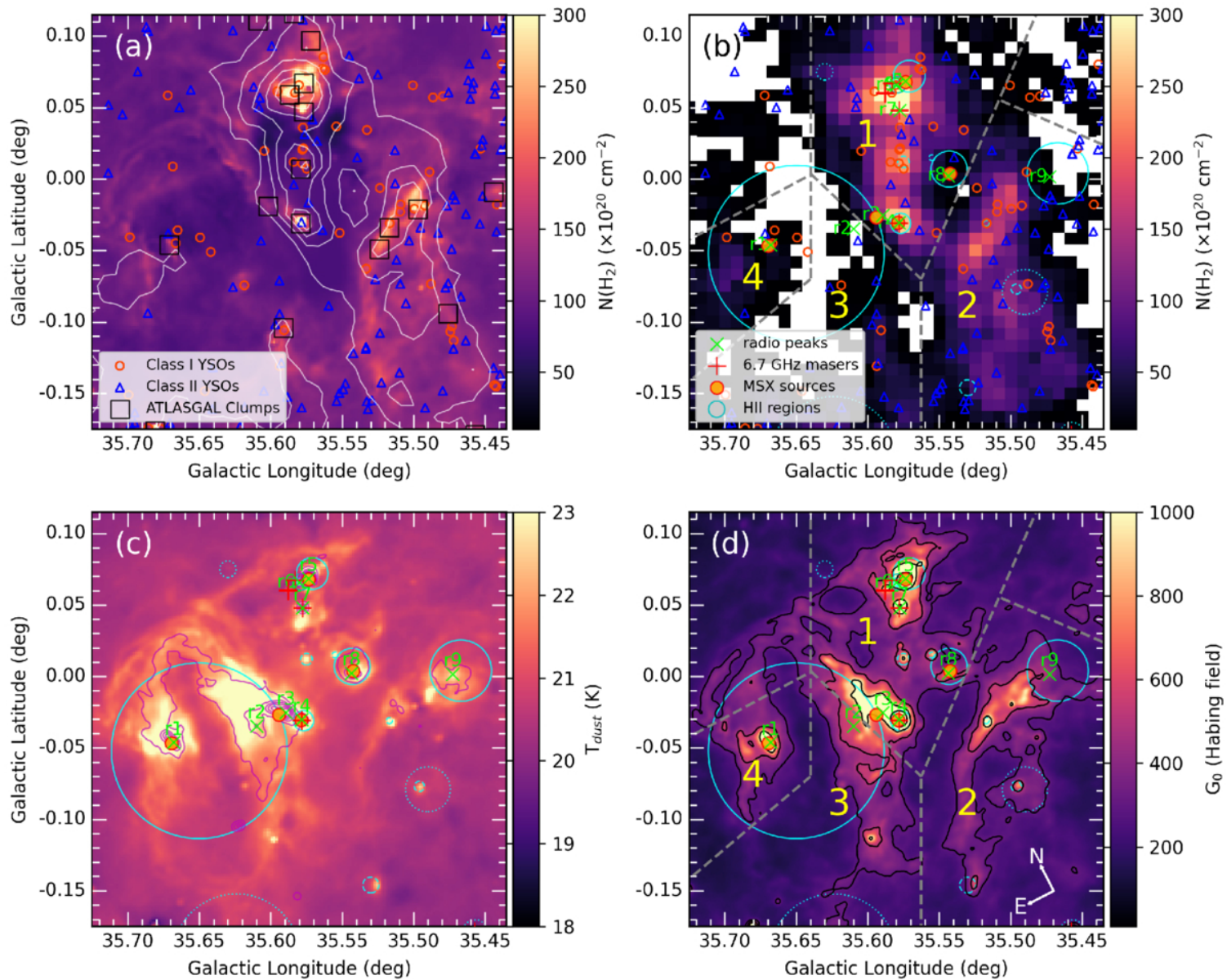
Figure 5. from En Chen and Xi Chen 2026 Astrophys. J. 1001 doi:10.3847/1538-4357/ae58a6 https://dx.doi.org/10.3847/1538-4357/ae58a6 © 2026. The Author(s). Published by the American Astronomical Society.
