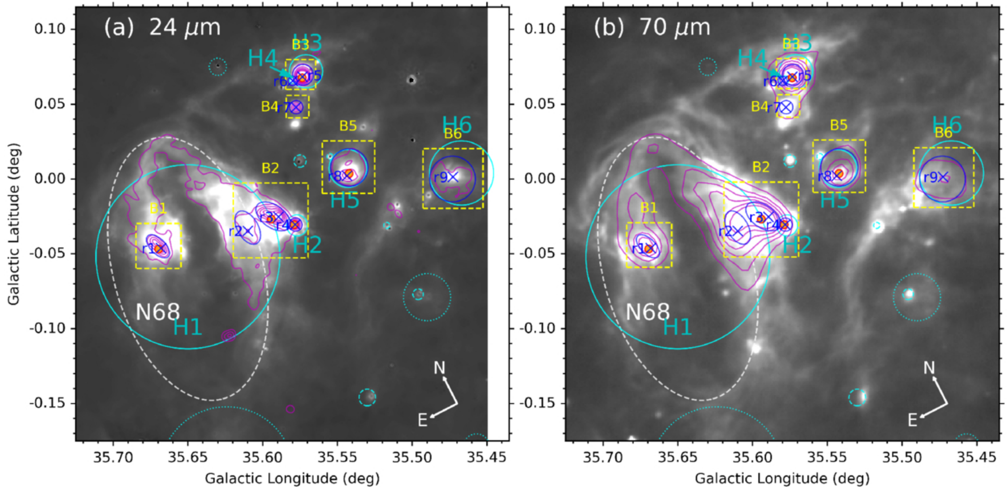
Figure 2. from En Chen and Xi Chen 2026 Astrophys. J. 1001 doi:10.3847/1538-4357/ae58a6 https://dx.doi.org/10.3847/1538-4357/ae58a6 © 2026. The Author(s). Published by the American Astronomical Society.
