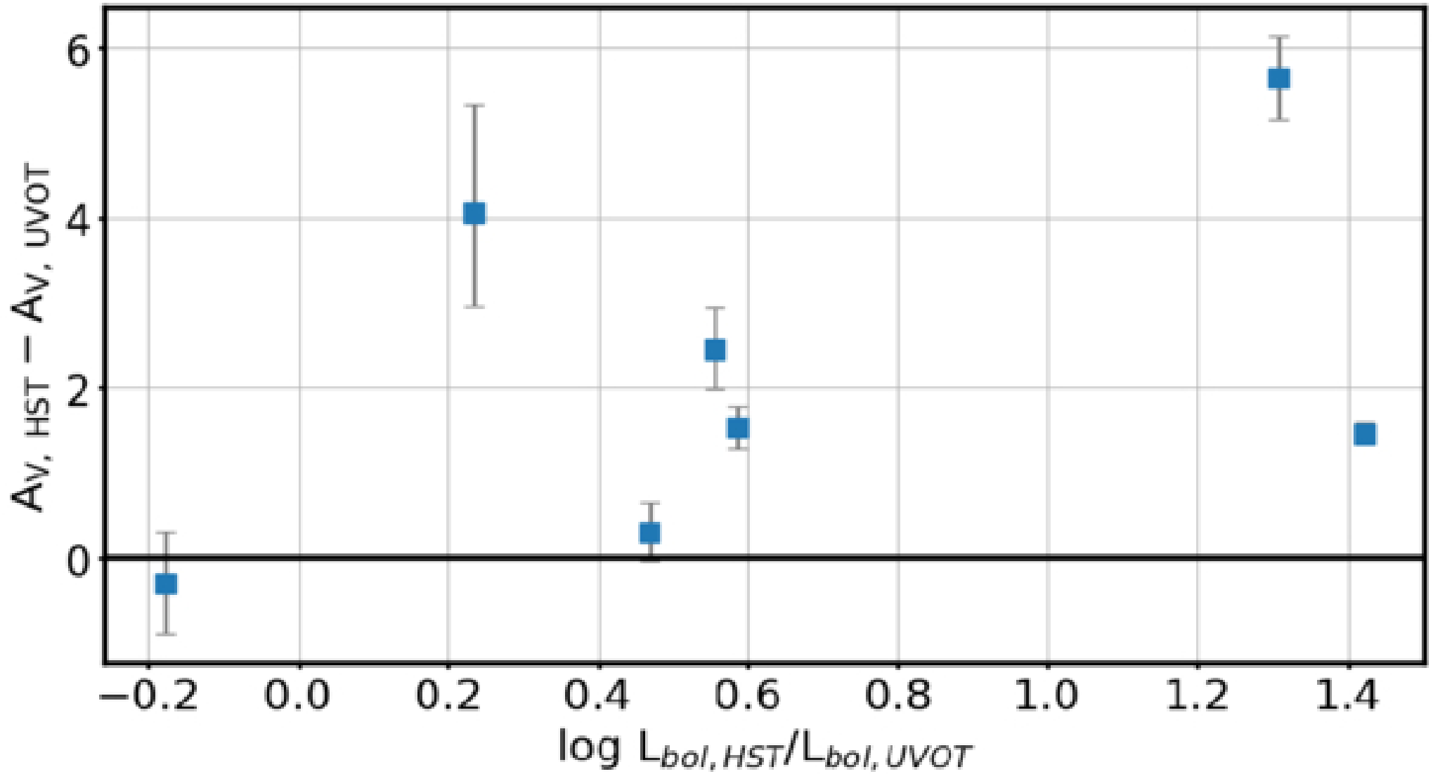
Figure 7. from Connor Auge et al 2026 Astrophys. J. 1002 doi:10.3847/1538-4357/ae581d https://dx.doi.org/10.3847/1538-4357/ae581d © 2026. The Author(s). Published by the American Astronomical Society.
