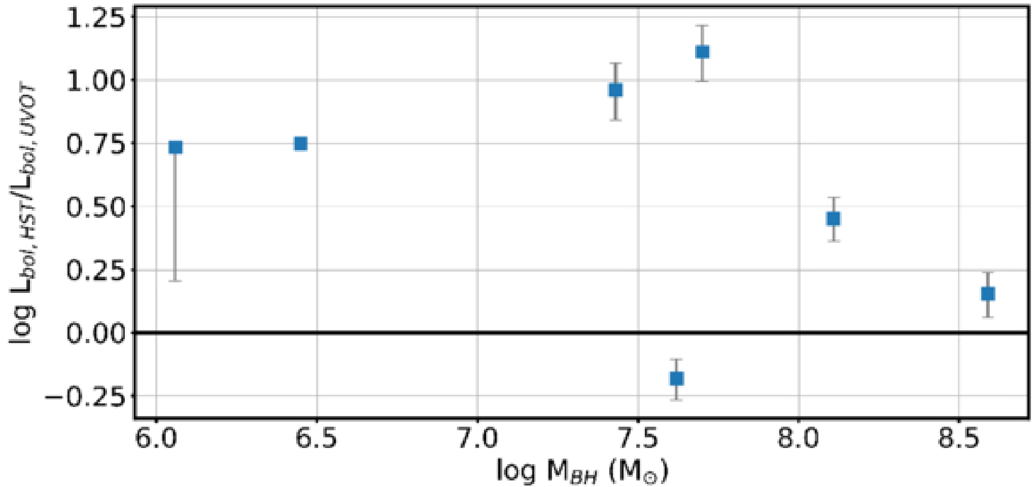
Figure 4. from Connor Auge et al 2026 Astrophys. J. 1002 doi:10.3847/1538-4357/ae581d https://dx.doi.org/10.3847/1538-4357/ae581d © 2026. The Author(s). Published by the American Astronomical Society.
