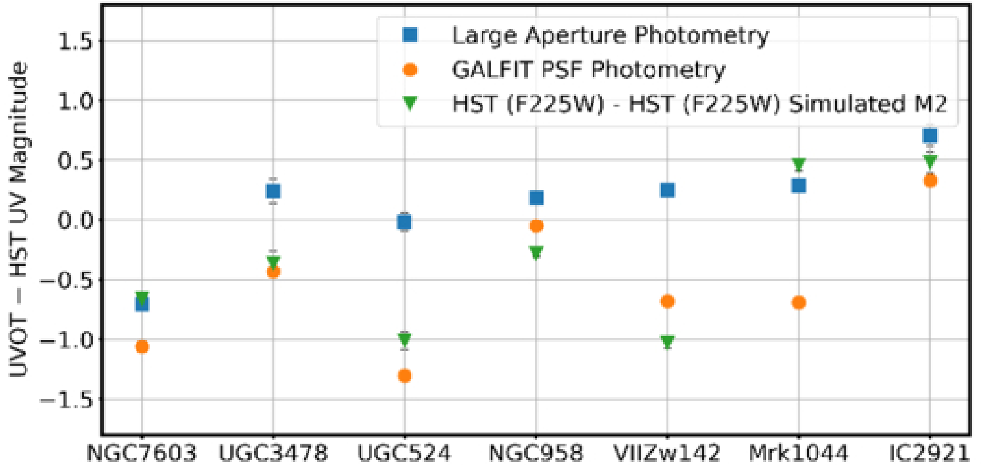
Figure 2. from Connor Auge et al 2026 Astrophys. J. 1002 doi:10.3847/1538-4357/ae581d https://dx.doi.org/10.3847/1538-4357/ae581d © 2026. The Author(s). Published by the American Astronomical Society.
