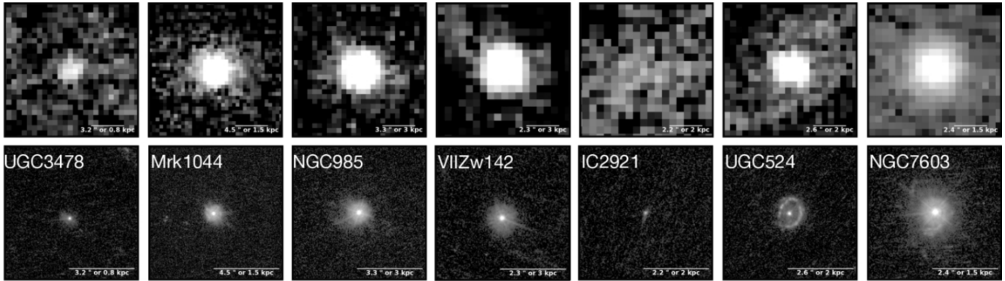
Figure 1. from Connor Auge et al 2026 Astrophys. J. 1002 doi:10.3847/1538-4357/ae581d https://dx.doi.org/10.3847/1538-4357/ae581d © 2026. The Author(s). Published by the American Astronomical Society.
