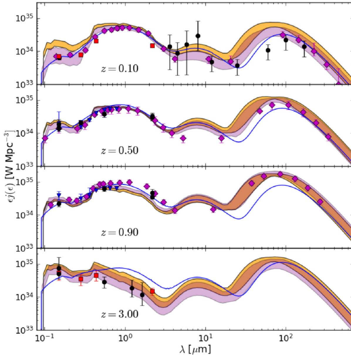
Figure 12. from Anuvab Banerjee et al 2026 Astrophys. J. 1003 doi:10.3847/1538-4357/ae581a https://dx.doi.org/10.3847/1538-4357/ae581a © 2026. The Author(s). Published by the American Astronomical Society.
