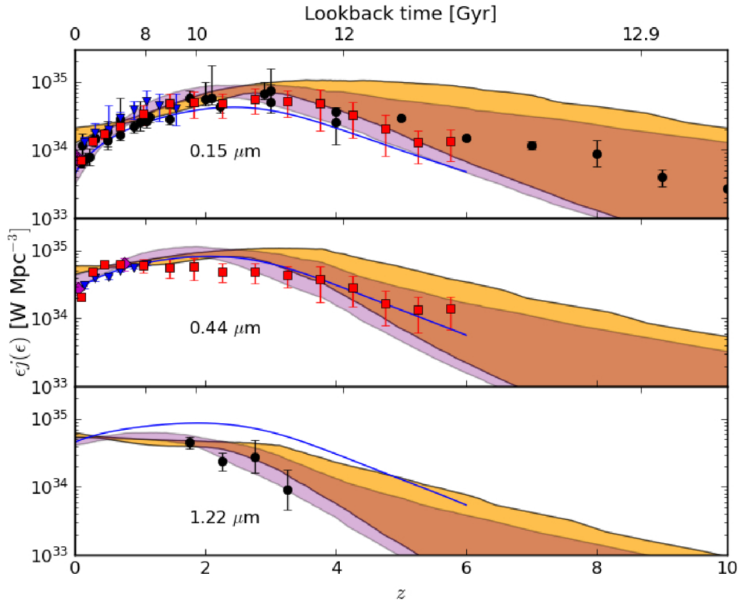
Figure 11. from Anuvab Banerjee et al 2026 Astrophys. J. 1003 doi:10.3847/1538-4357/ae581a https://dx.doi.org/10.3847/1538-4357/ae581a © 2026. The Author(s). Published by the American Astronomical Society.
