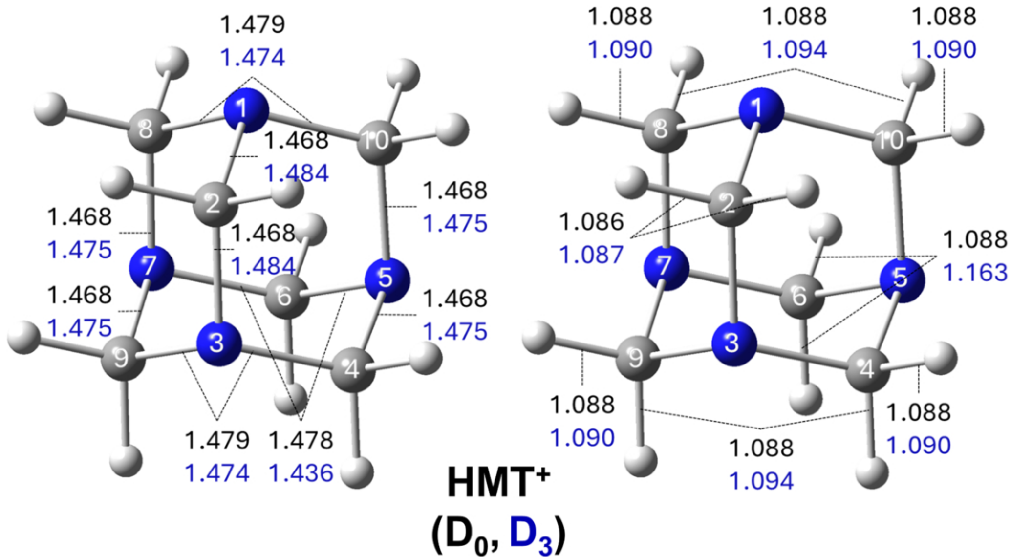
Figure 6. from Parker Crandall et al 2026 Astrophys. J. 1001 doi:10.3847/1538-4357/ae5811 https://dx.doi.org/10.3847/1538-4357/ae5811 © 2026. The Author(s). Published by the American Astronomical Society.
