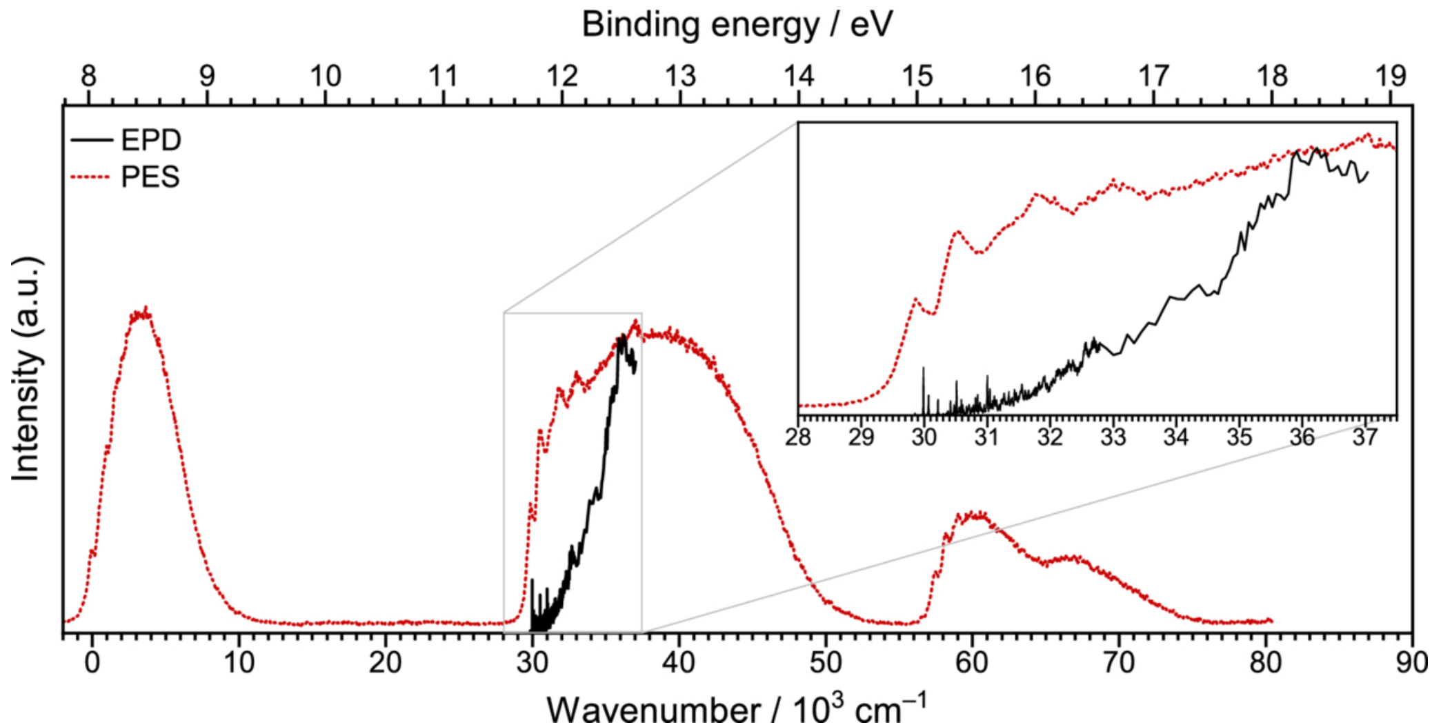
Figure 4. from Parker Crandall et al 2026 Astrophys. J. 1001 doi:10.3847/1538-4357/ae5811 https://dx.doi.org/10.3847/1538-4357/ae5811 © 2026. The Author(s). Published by the American Astronomical Society.
