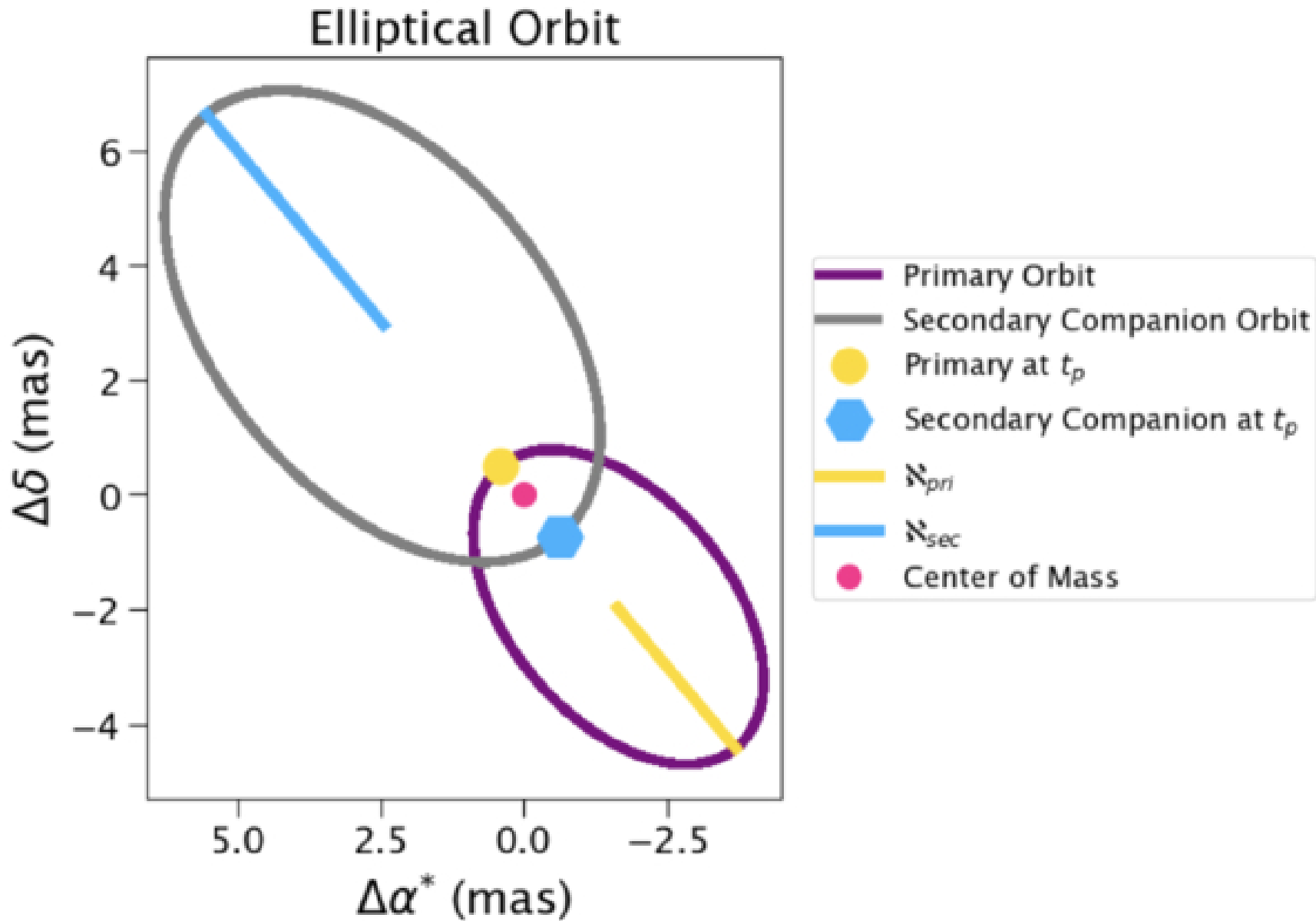
Figure 2. from T. Dex Bhadra et al 2026 Astrophys. J. 1002 doi:10.3847/1538-4357/ae5701 https://dx.doi.org/10.3847/1538-4357/ae5701 © 2026. The Author(s). Published by the American Astronomical Society.
