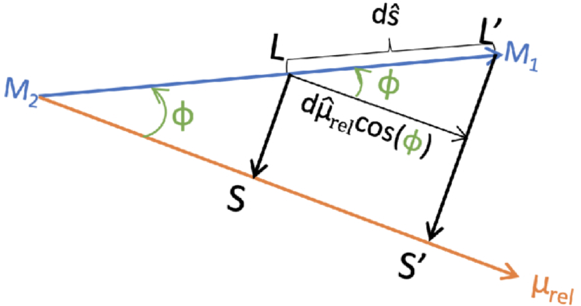
Figure 19. from T. Dex Bhadra et al 2026 Astrophys. J. 1002 doi:10.3847/1538-4357/ae5701 https://dx.doi.org/10.3847/1538-4357/ae5701 © 2026. The Author(s). Published by the American Astronomical Society.
