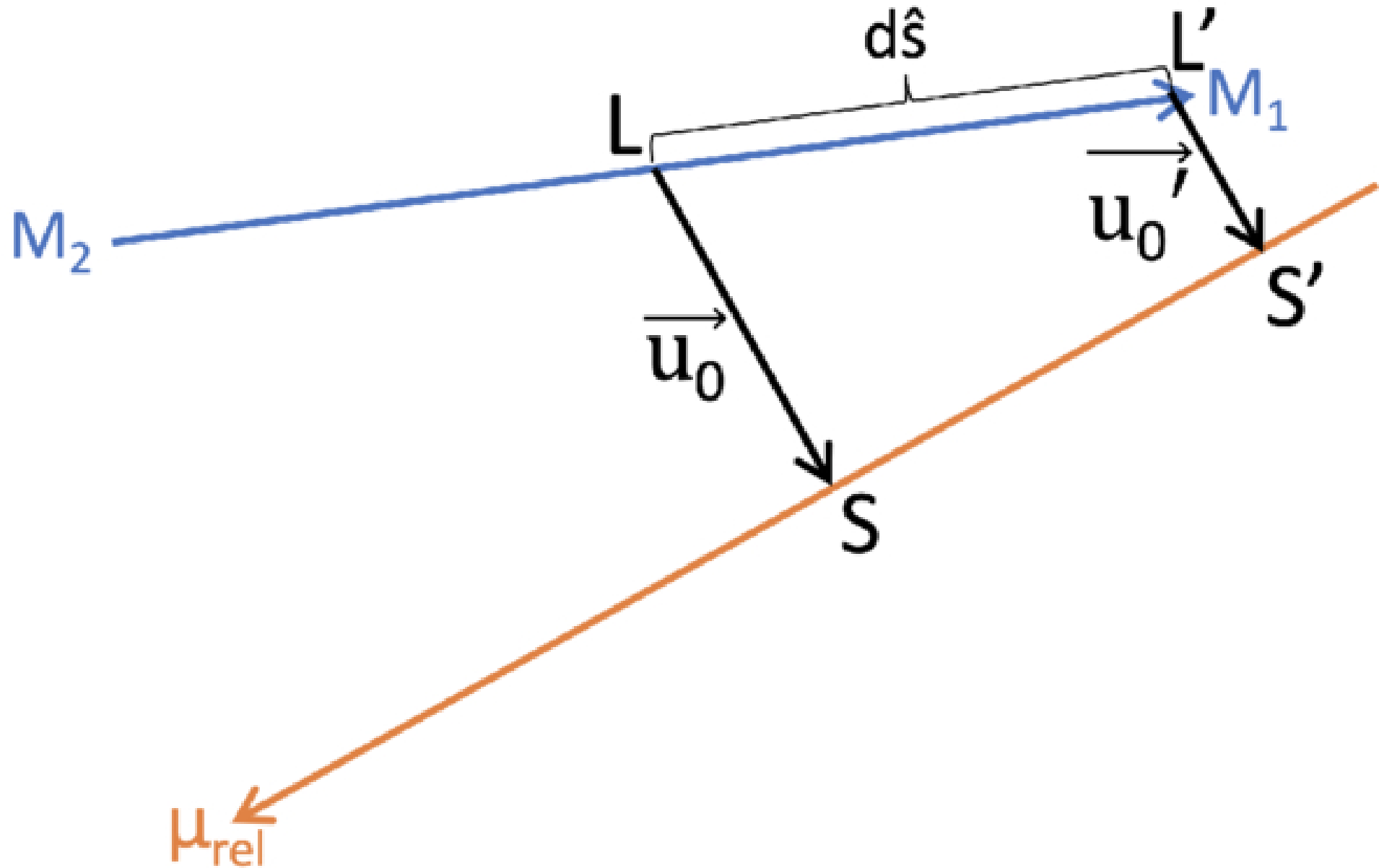
Figure 18. from T. Dex Bhadra et al 2026 Astrophys. J. 1002 doi:10.3847/1538-4357/ae5701 https://dx.doi.org/10.3847/1538-4357/ae5701 © 2026. The Author(s). Published by the American Astronomical Society.
