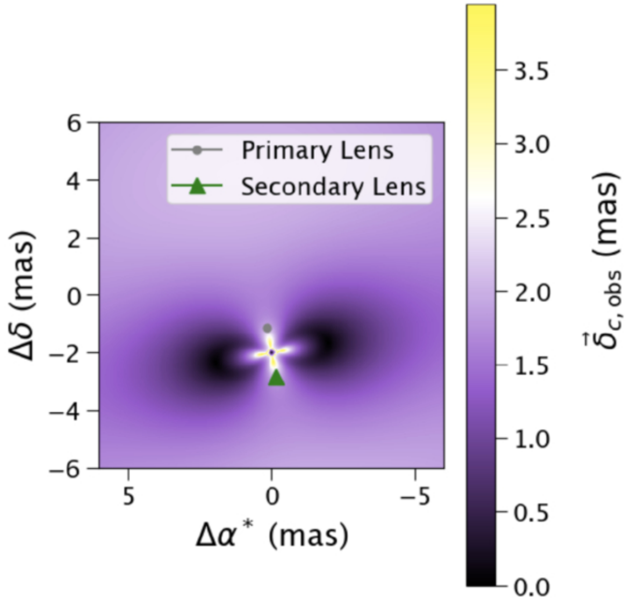
Figure 12. from T. Dex Bhadra et al 2026 Astrophys. J. 1002 doi:10.3847/1538-4357/ae5701 https://dx.doi.org/10.3847/1538-4357/ae5701 © 2026. The Author(s). Published by the American Astronomical Society.
