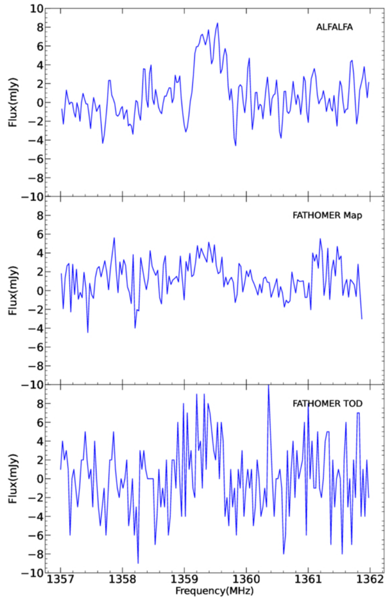
Figure 9. from Shuanghao Shu et al 2026 Astrophys. J. 1001 doi:10.3847/1538-4357/ae56f6 https://dx.doi.org/10.3847/1538-4357/ae56f6 © 2026. The Author(s). Published by the American Astronomical Society.
