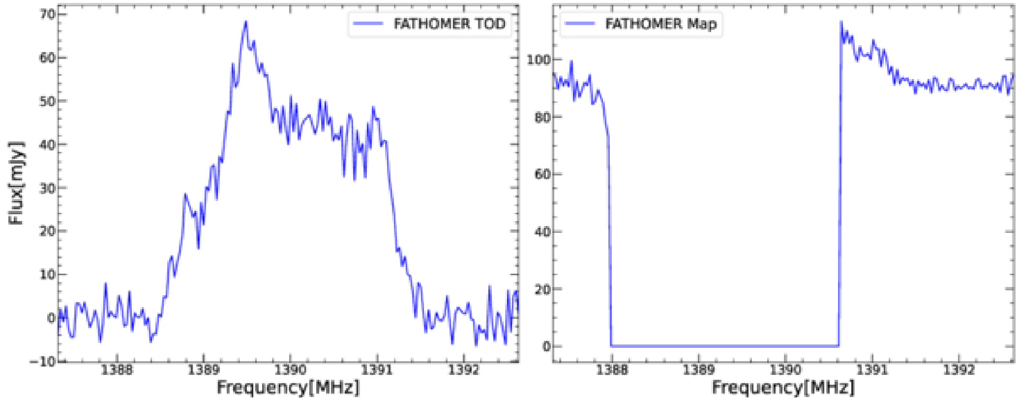
Figure 12. from Shuanghao Shu et al 2026 Astrophys. J. 1001 doi:10.3847/1538-4357/ae56f6 https://dx.doi.org/10.3847/1538-4357/ae56f6 © 2026. The Author(s). Published by the American Astronomical Society.
