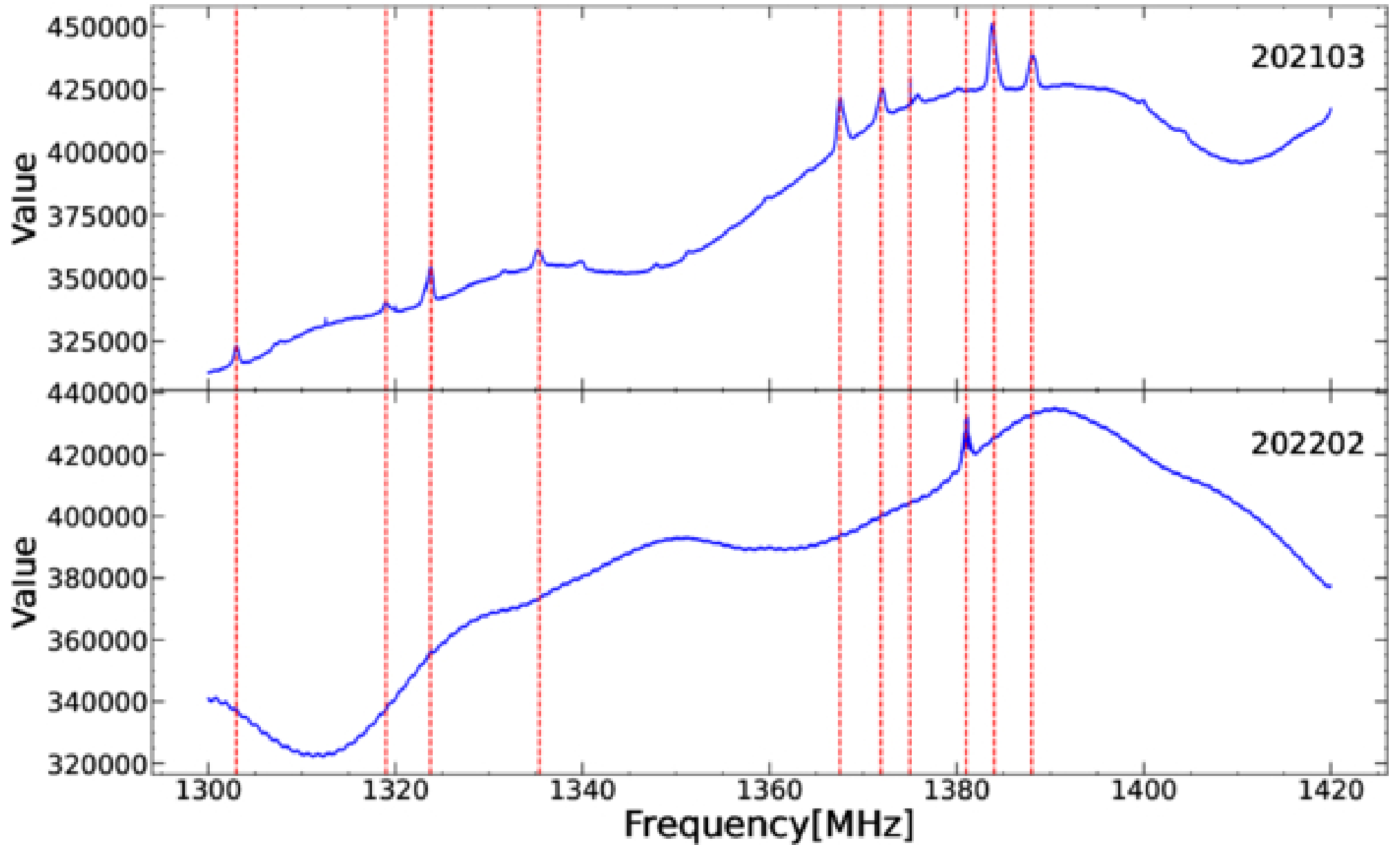
Figure 10. from Shuanghao Shu et al 2026 Astrophys. J. 1001 doi:10.3847/1538-4357/ae56f6 https://dx.doi.org/10.3847/1538-4357/ae56f6 © 2026. The Author(s). Published by the American Astronomical Society.
