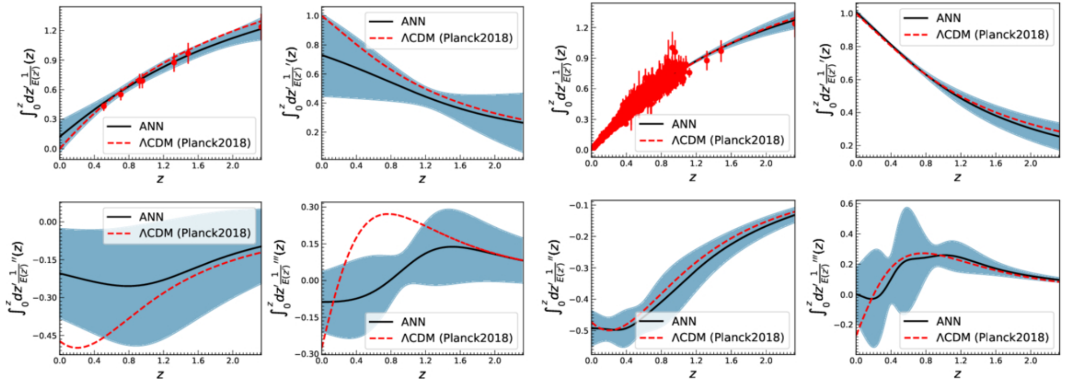
Figure 4. from Qile Zhang et al 2026 Astrophys. J. 1002 doi:10.3847/1538-4357/ae56f5 https://dx.doi.org/10.3847/1538-4357/ae56f5 © 2026. The Author(s). Published by the American Astronomical Society.
