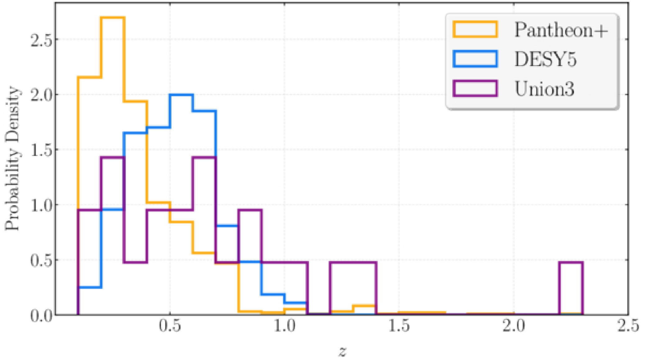
Figure 1. from Qile Zhang et al 2026 Astrophys. J. 1002 doi:10.3847/1538-4357/ae56f5 https://dx.doi.org/10.3847/1538-4357/ae56f5 © 2026. The Author(s). Published by the American Astronomical Society.
