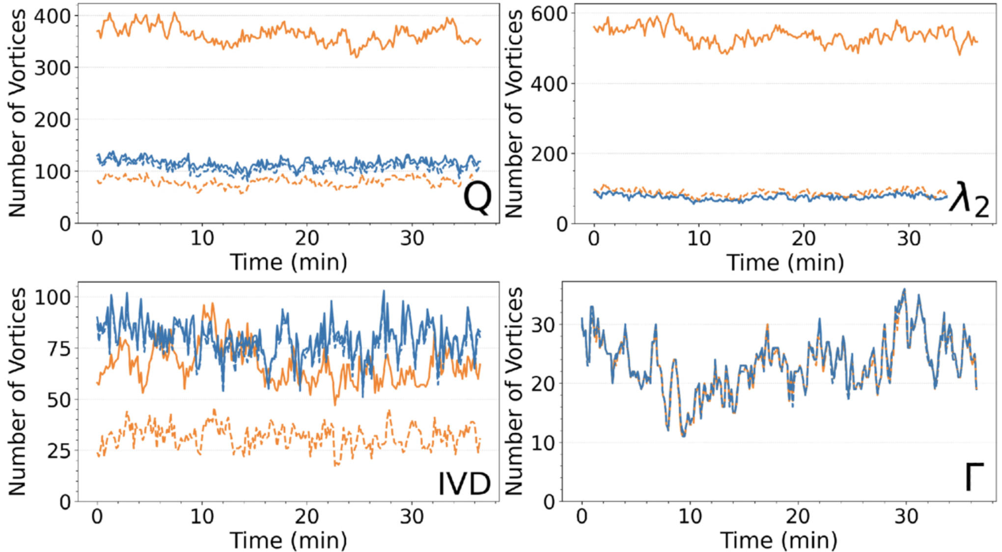
Figure 3. from Lauren McClure et al 2026 Astrophys. J. 1002 doi:10.3847/1538-4357/ae56f4 https://dx.doi.org/10.3847/1538-4357/ae56f4 © 2026. The Author(s). Published by the American Astronomical Society.
