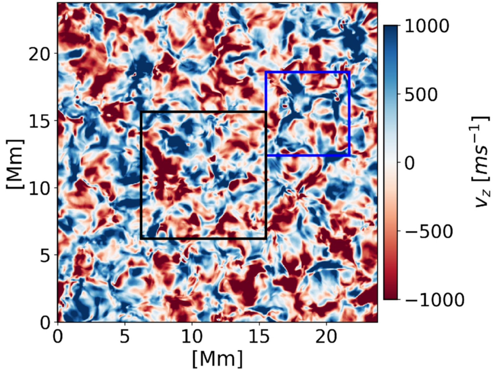
Figure 1. from Lauren McClure et al 2026 Astrophys. J. 1002 doi:10.3847/1538-4357/ae56f4 https://dx.doi.org/10.3847/1538-4357/ae56f4 © 2026. The Author(s). Published by the American Astronomical Society.
