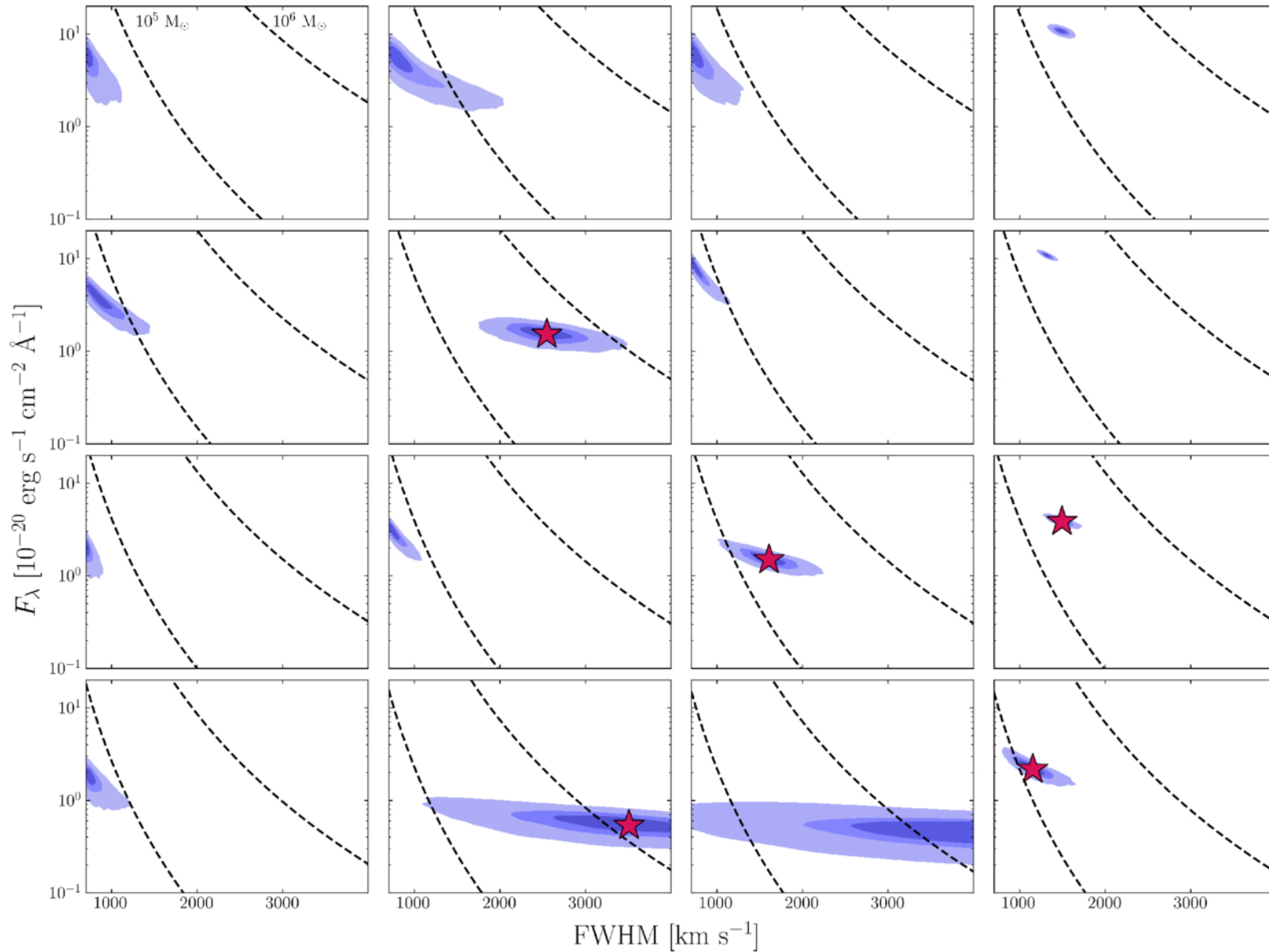
Figure 4. from Madisyn Brooks et al 2026 Astrophys. J. 1002 doi:10.3847/1538-4357/ae5652 https://dx.doi.org/10.3847/1538-4357/ae5652 © 2026. The Author(s). Published by the American Astronomical Society.
