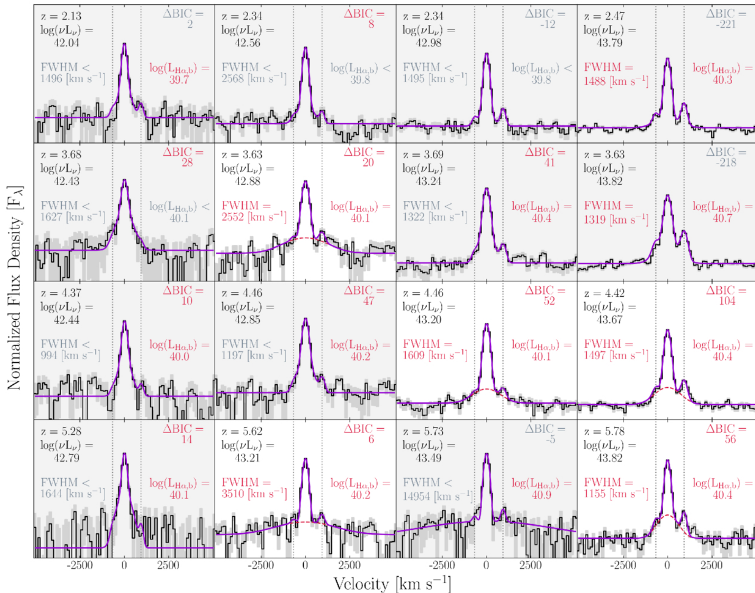
Figure 2. from Madisyn Brooks et al 2026 Astrophys. J. 1002 doi:10.3847/1538-4357/ae5652 https://dx.doi.org/10.3847/1538-4357/ae5652 © 2026. The Author(s). Published by the American Astronomical Society.
