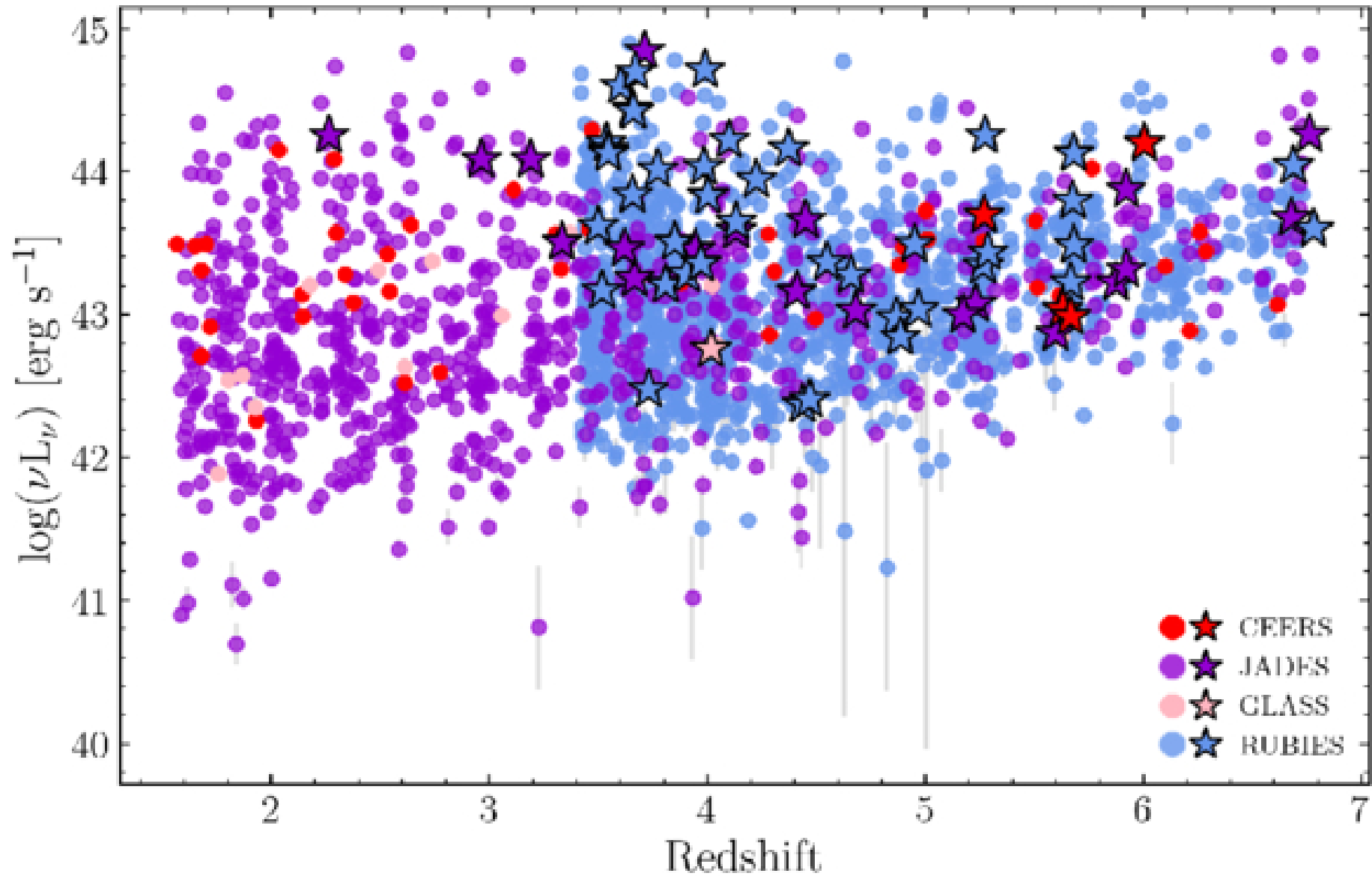
Figure 1. from Madisyn Brooks et al 2026 Astrophys. J. 1002 doi:10.3847/1538-4357/ae5652 https://dx.doi.org/10.3847/1538-4357/ae5652 © 2026. The Author(s). Published by the American Astronomical Society.
