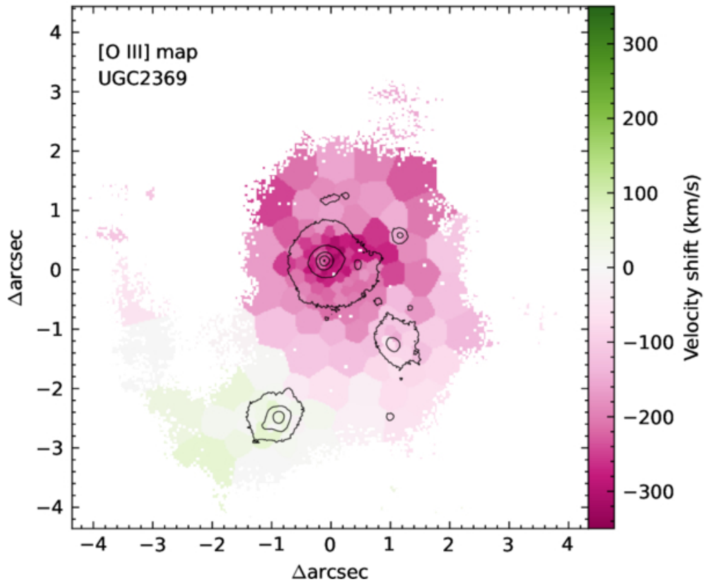
Figure 6. from Yuanze Ding et al 2026 Astrophys. J. 1002 doi:10.3847/1538-4357/ae5643 https://dx.doi.org/10.3847/1538-4357/ae5643 © 2026. The Author(s). Published by the American Astronomical Society.
